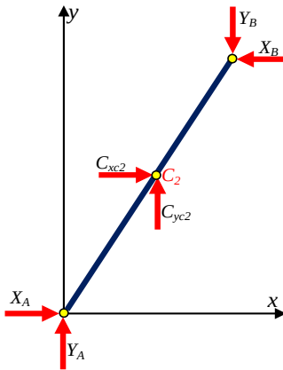
Fig. 9. Linkage I—Equilibrium conditions for the point AB
